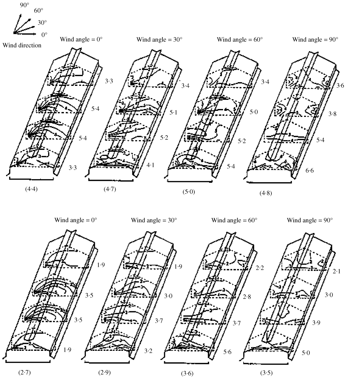
Fig. 5. Spatial distribution of temperature rise in ^{\circ}\text{C} with changing wind direction at reference wind velocities of 1.0\text{ m s}^{-1} (upper) and 4.6\text{ m s}^{-1} (lower) measured in wind tunnel testing of model scale 1/10 greenhouse. The value on the right of each transverse section and the value in parenthesis denote the average temperature in the crop space of the section and the average over four sections, respectively (after Sase et al. , 1984)
