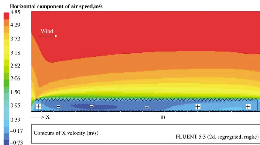
Fig. 12. Predicted X -velocity distribution in and around a 60 span Venlo-type glasshouse under leeward ventilation with a reference velocity at ridge height of 3.5 \text{ m s}^{-1} and using a renormalisation group (RNG) turbulence model. The total spans are schematised along the X -axis and the signs + or – in the figure refer to the areas within the greenhouse space with a positive or negative X -velocity. The point D indicate the place where the flux is reversed (after Reichrath & Davies, 2001)
